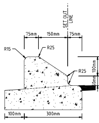
GAP KERB DETAILS NTS
