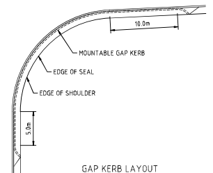
GAP KERB LAYOUT NTS
